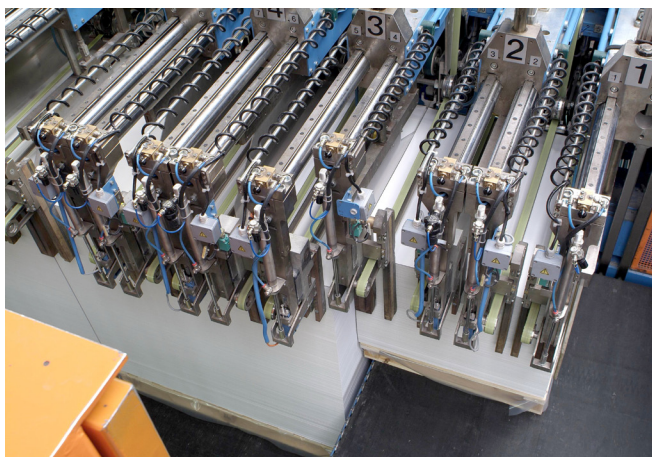
Auto positioning of side joggers and backstops for simplex and duplex formats.
